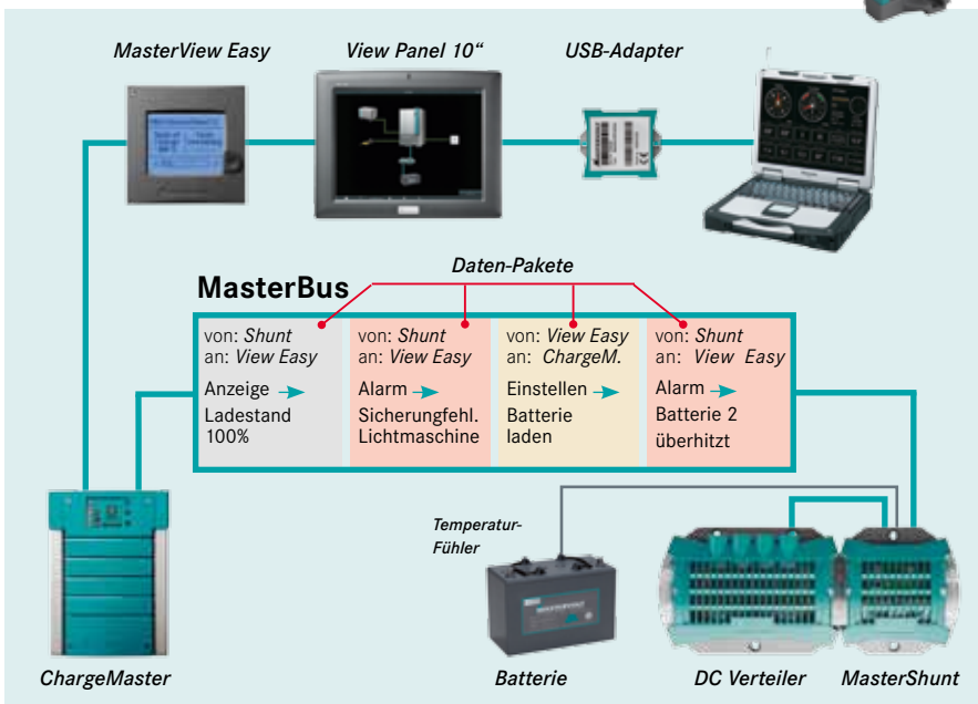
MasterShunt 500
